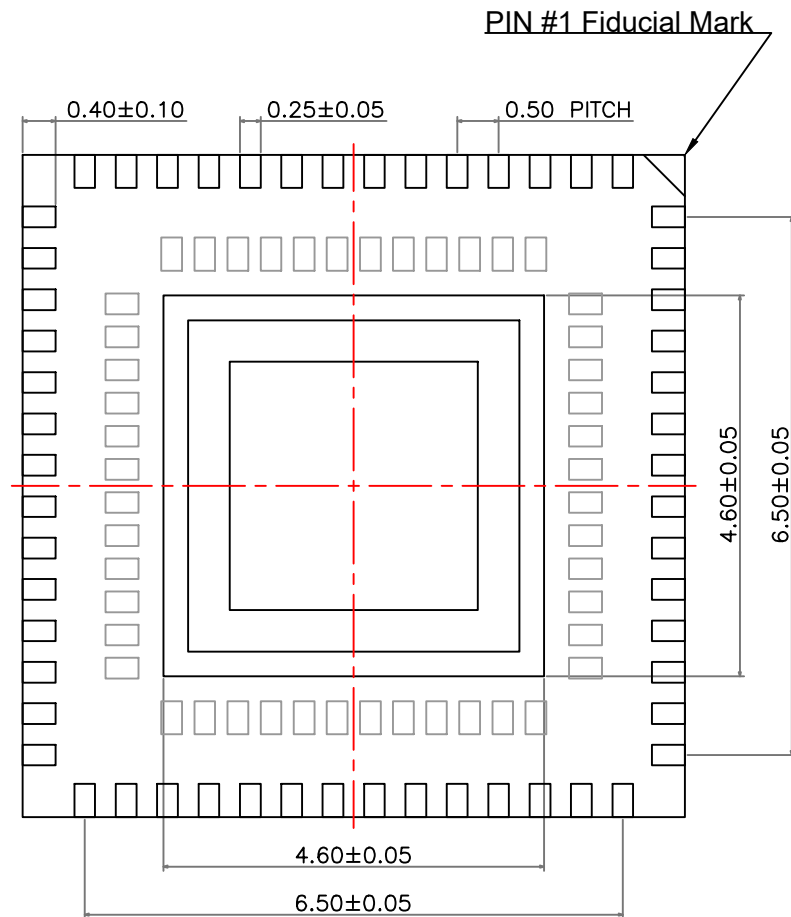
BOTTOM VIEW
